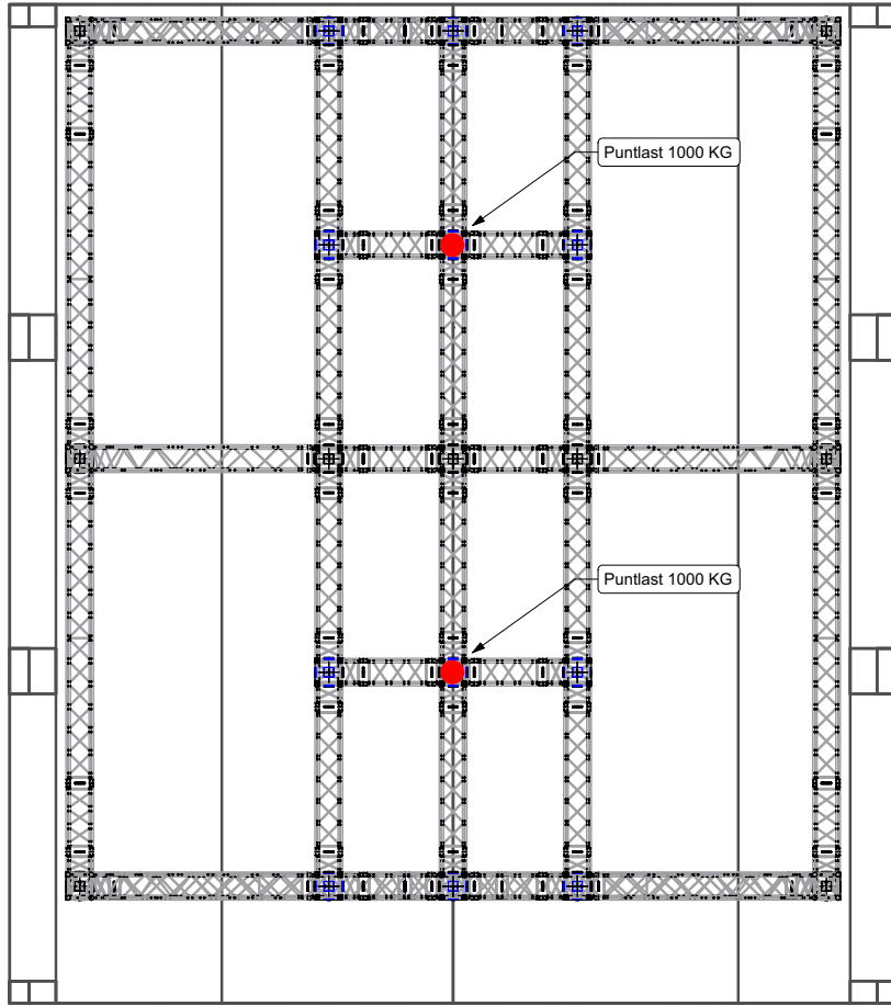
2-Puntsbelasting
